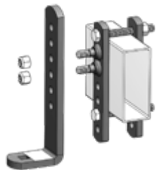
Figure 15 - Initial position for top-mounted coupler.
