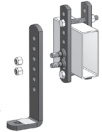
Figure 15 - Setup for bottom-mounted coupler.
